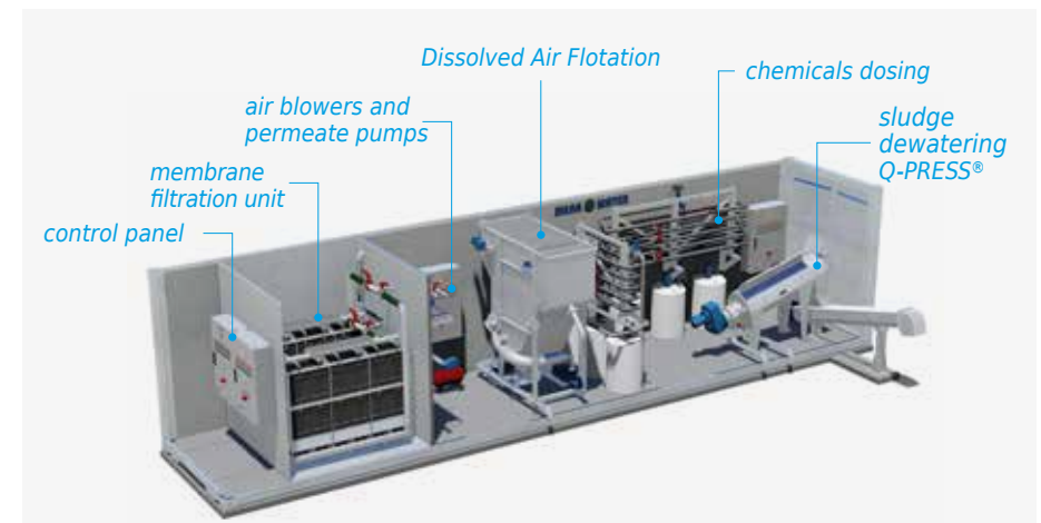
Package plants for industrial wastewater treatment.
